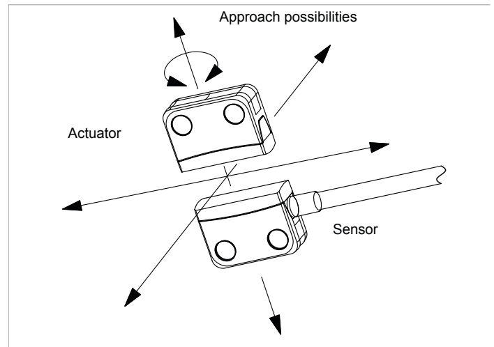
Figure 3: Control possibilities
