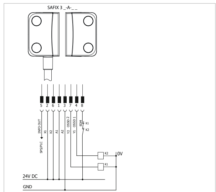
Figure 5: Connection with diagnosis output, automatic reset Automatic for the EDM input variation (SAFIX _-A-_ _) The inputs X1 and X2 are supplied with 24 V DC. The outputs Y1 and Y2 are included in the analysis. The diagnosis output can be connected, for example, to an SPS.
