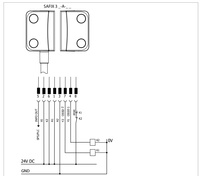
Figure 5: Connection with diagnosis output, automatic reset Automatic for the EMD input variation (SAFIX __-A-__)
