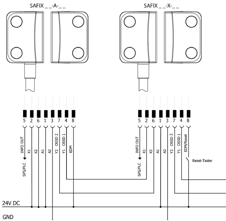
Figure 8: Input from a reset button + every door circuit can be acknowledged, SAFIX __-X-__ Series connection of multiple SAFIX sensors with manual reset. The reset button always has to be connected to the last sensor. (SAFIX __-X-__) All other sensors must be used with the automatic start variation (SAFIX __-A-__)
