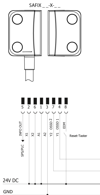
Figure 7: Input from a reset button Monitored for the EMD input variation (SAFIX __-X-__) The inputs X1 and X2 are supplied with 24 V DC. The outputs Y1 and Y2 are included in the analysis. The diagnosis output can be connected, for example, to an SPS. The input EDM waits for a start pulse duration between 30 ms and 5 s.
